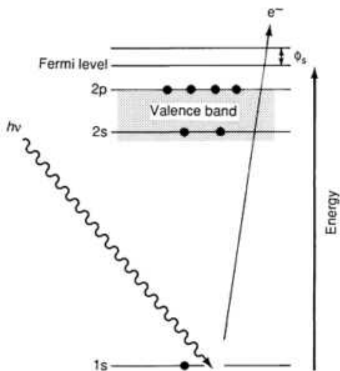
Fig. 1 Photoelectric effect
