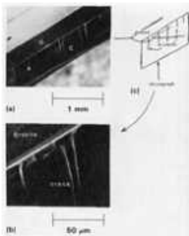
Fig. 6 Cross section of dicing groove in p -type silicon. (a) Scanning electron micrograph of groove (G) and subsurface cracks. (b) Close-up view. (c) Schematic showing location of subsurface damage beneath groove
