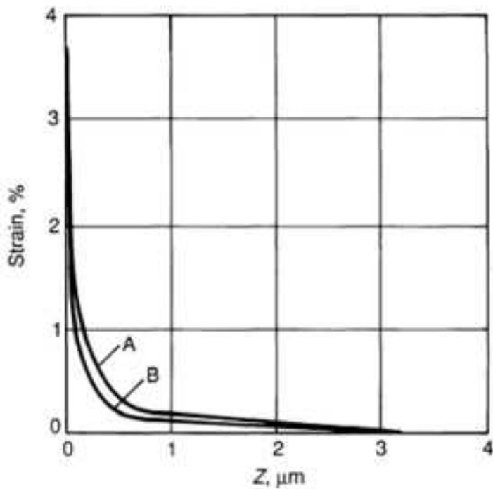
Fig. 9 Depth profiles of strain for ground sample obtained with symmetrical optics. A, \text{CuK}\alpha radiation; B, \lambda = 0.24797 \text{ nm} (synchrotron radiation). Source: Ref 15
