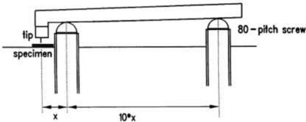
Fig. 2 Example of coarse approach using fine-thread screws and mechanical advantage of a cantilever beam
