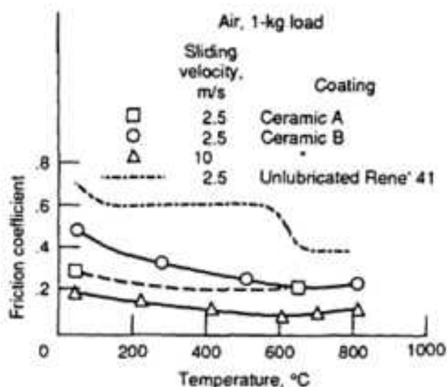
Fig. 20 Friction-temperature characteristics of fluoride coatings modified with silicate and oxide additions. Ceramic A: 60.8\text{CaF}_2 - 13.1\text{LiF} - 17.4\text{Ca}_2\text{SiO}_4 - 8.7\text{CaO} . Ceramic B: 48.3\text{BaF}_2 - 21.7\text{CaF}_2 - 20\text{Ca}_2\text{SiO}_4 - 10\text{CaO}
