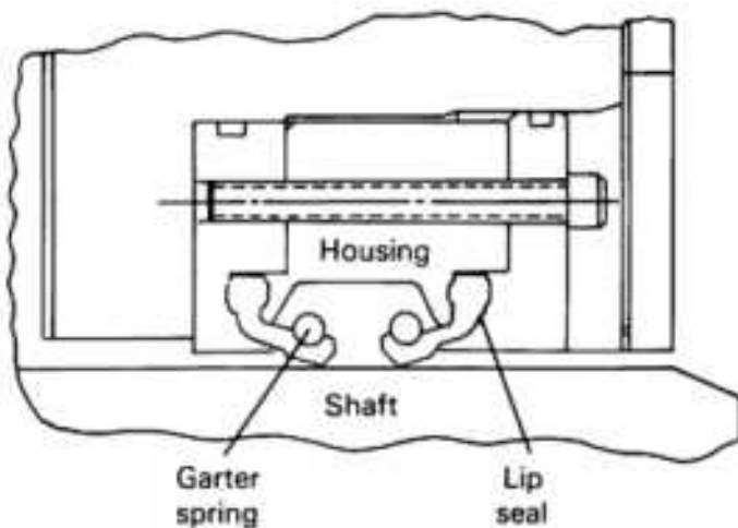
Fig. 3 Lip seal
