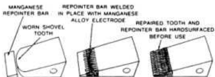
Fig. 13 Worn shovel tooth often rebuilt by welding a new repointer bar, usually made of high-manganese steel, onto end of tooth prior to depositing hardfacing materials. Source: Ref 32
