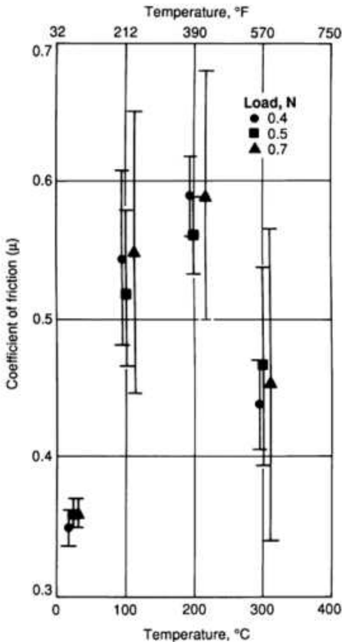
Fig. 10 Plot of the dynamic coefficient of friction versus temperature for (100) n -type silicon (electrical resistivity, \rho , of 3.3\ \Omega\cdot\text{cm} ) abraded by a Vickers pyramidal diamond at selected loads.
