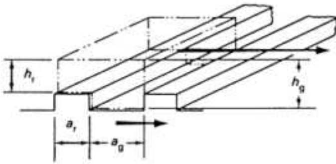
Fig. 24 Geometry of spiral-groove bearing, using notation of Castelli and Vohr (Ref 28)
