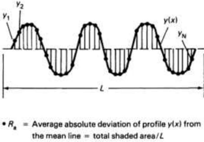
Fig. 1 Idealized stylus profile showing the mean line; the evaluation length, L ; the digitized points, y_i ; and a definition of the parameter R_a
