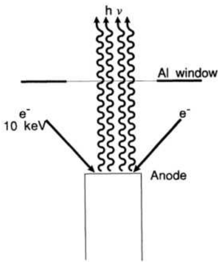
Fig. 3 Typical x-ray source, where electrons are accelerated to about 10 keV to the anode material, which then emits photons with energy characteristic of the anode material
