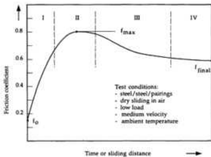
Fig. 1 A friction-time master curve
