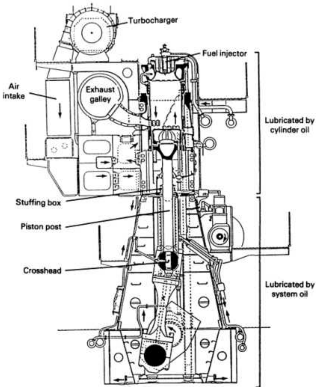
Fig. 7 Cross section of crosshead marine diesel engine. Source: Ref 16
