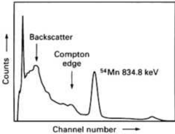
Fig. 12 Typical gamma spectrum for 54 Mn
