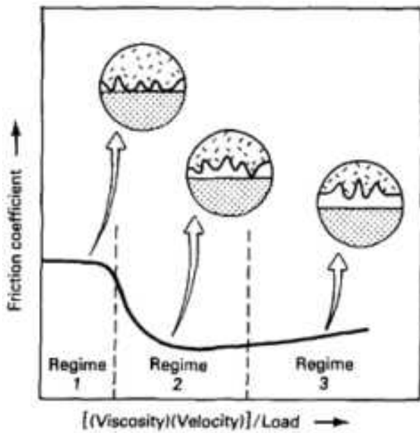
Fig. 1 Plot of friction coefficient, \mu versus [(\text{viscosity})(\text{velocity})]/\text{load} , (\eta_0 U)/P , to show range of the three regimes of lubrication. Regime 1, boundary lubrication; regime 2, thin-film lubrication; regime 3, thick-film lubrication
