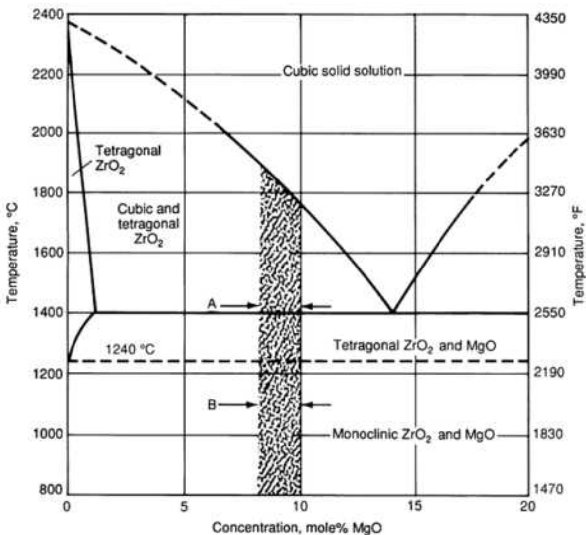
Fig. 4 Zirconia \text{MgO} phase diagram. The shaded region indicates the composition range used in most commercially available alloys. Aging is carried out at temperatures above the eutectoid temperature at A to obtain maximum strength and below the eutectoid temperature at B to obtain maximum thermal shock resistance.
