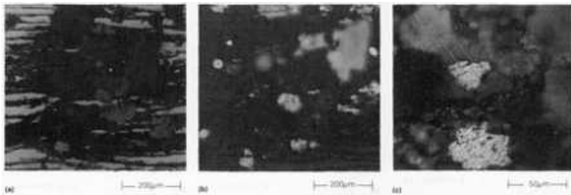
Fig. 7 Gearbox wear. (a) Wear particles resulting from gear overload. 100 \times . (b) Red oxide particles. Polarized reflected light. 100 \times . (c) Temper-colored particles. 400 \times
