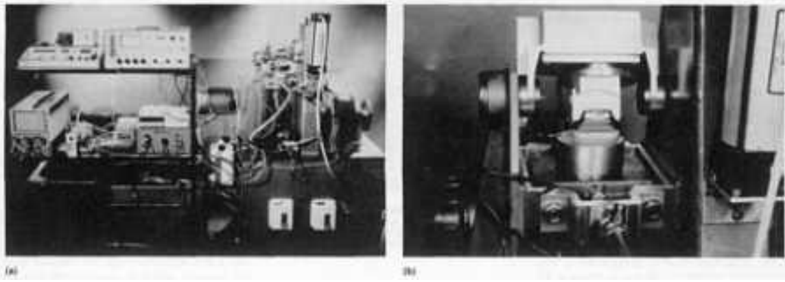
Fig. 9 Knee joint simulator used to evaluate magnitude and distribution of wear in a total replacement knee joint. (a) Complete machine setup showing test apparatus and accompanying state-of-the-art monitoring/recording instrumentation. (b) Closeup view of test cell showing knee joint implant being evaluated while it is held in position in a test fixture
