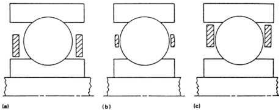
Fig. 17 Schematic showing types of rolling bearing cages. (a) Inner ringland riding. (b) Ball riding. (c) Outer ringland riding
