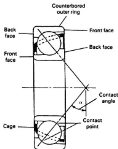
Angular-contact bearing.
