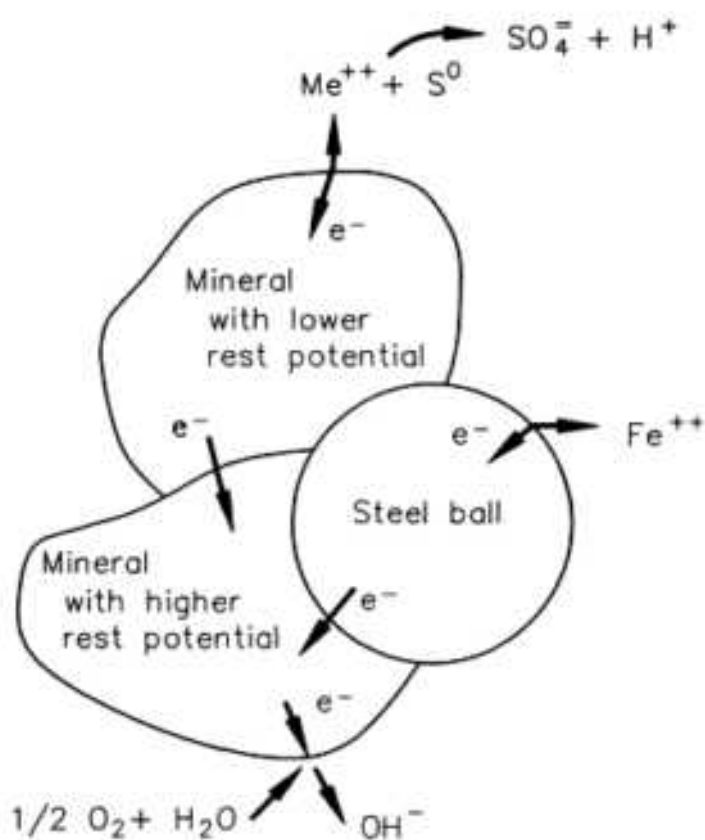
Fig. 13 Model of galvanic interactions among two minerals and grinding media. Source: Ref 39
