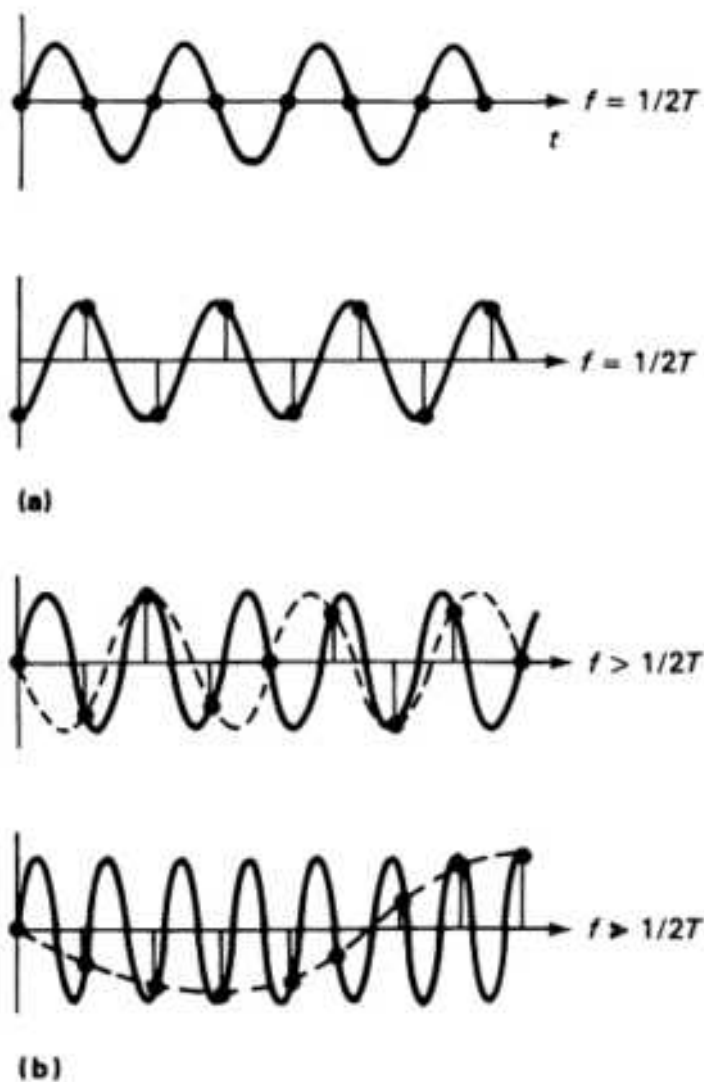
Fig. 3 Examples of aliasing. (a) Extraction of useful information not possible. f , frequency; T , time period in seconds. (b) Frequency created that does not exist in original data
