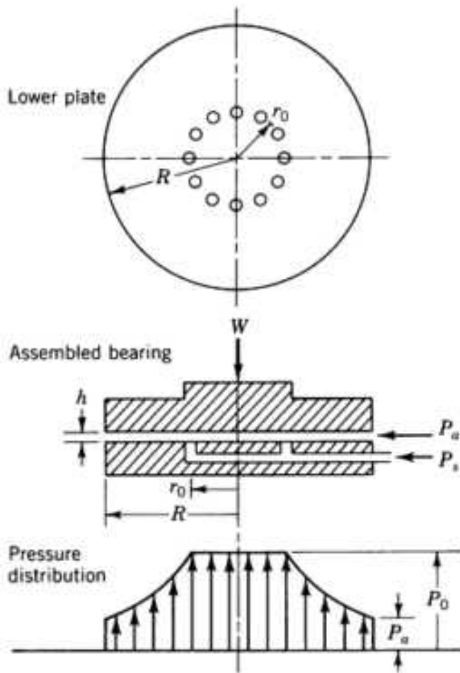
Fig. 30 Multiple-source feed for thrust bearing
