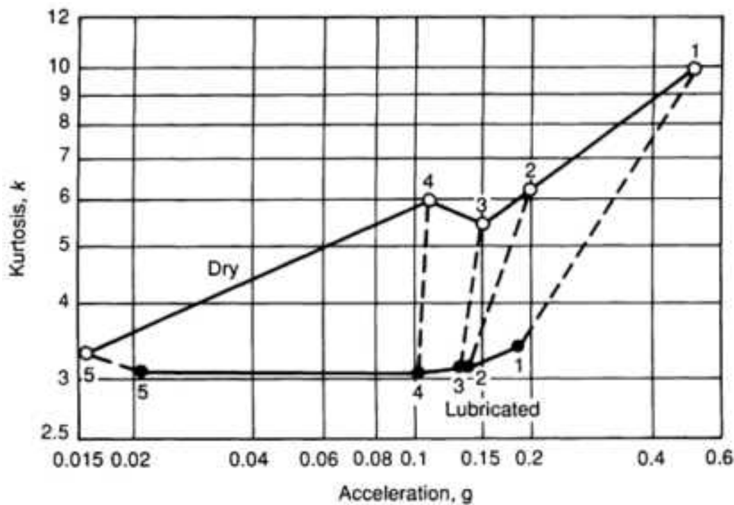
Fig. 9 Difference between dry and lubricating bearing. Points labeled 1 indicate frequency range from 2.5 to 5 kHz; points 2, 5 to 10 kHz; points 3, 10 to 20 kHz; points 4, 20 to 40 kHz; points 5, 40 to 80 kHz
