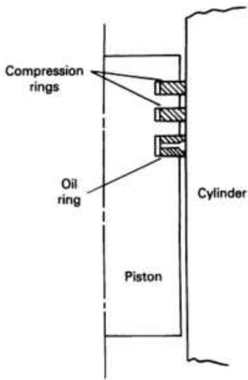
Fig. 7 Schematic of piston ring assembly showing location of compression rings and oil ring
