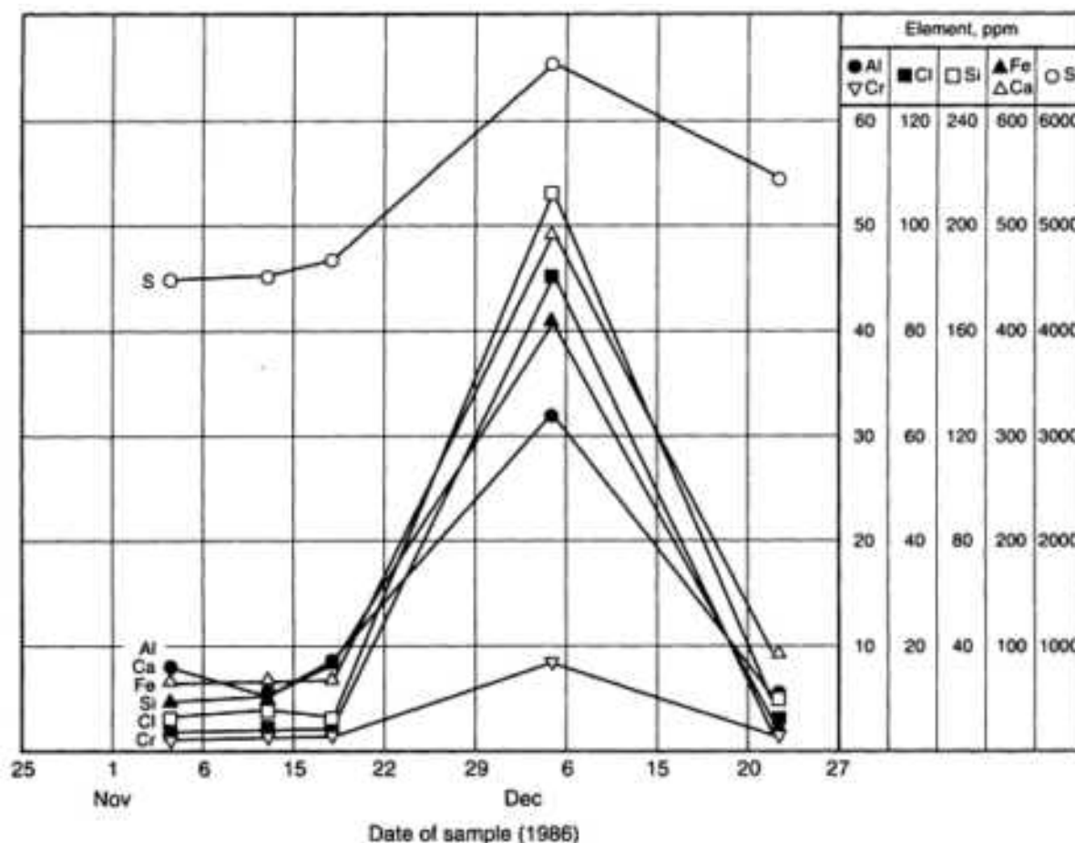
Fig. 11 Spectrophraphic analysis of metals in lubricant samples from a P-975 moist solvent pump before and after failure
