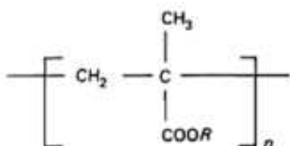
Alkyl polymethacrylate
