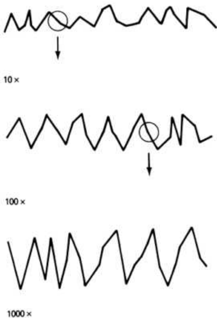
Fig. 11 Self-affine fractal
