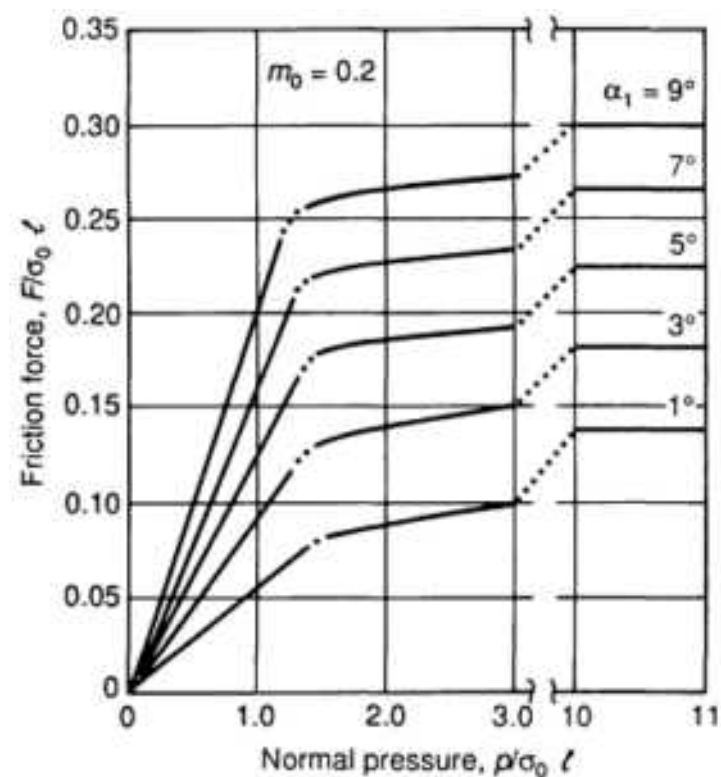
Fig. 21 The relation between the friction force and normal pressure with wedge angle ( \alpha_1 ) as a parameter
