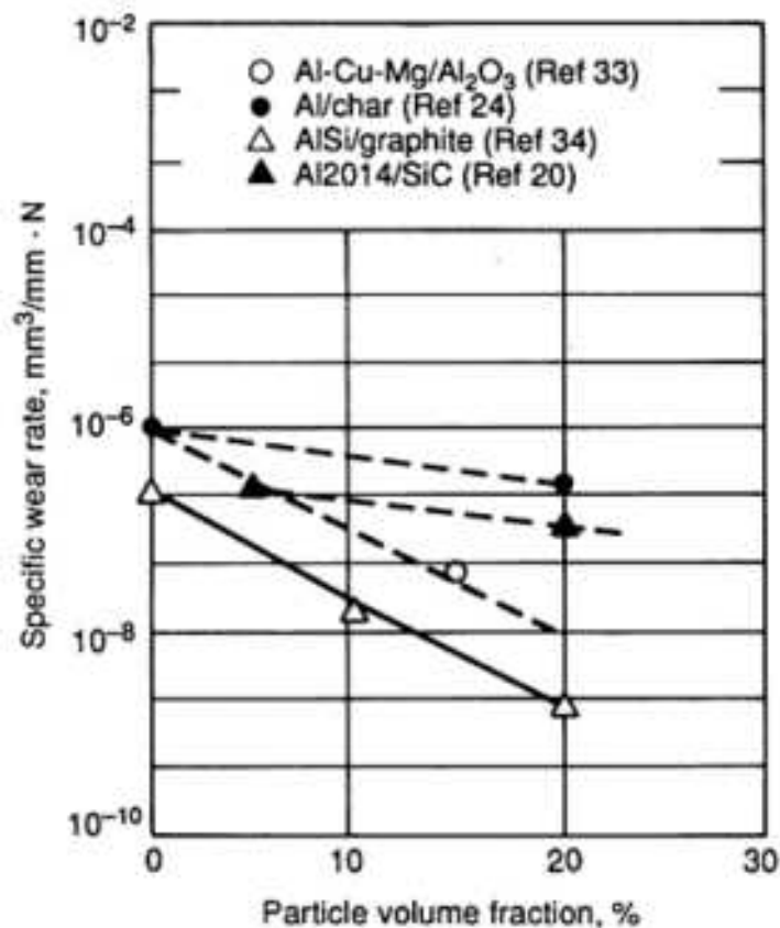
Fig. 5 Specific wear rates for several aluminum alloy particulate composites sliding against steel as a function of particle volume fraction
