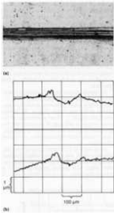
Fig. 13 (a) Portion of wear scar on flat, high-purity iron specimen tested in reciprocal sliding; magnification: 45×. (b) Two examples of cross-sectional surface profiles of scar at different locations, which can be used to measure wear area
