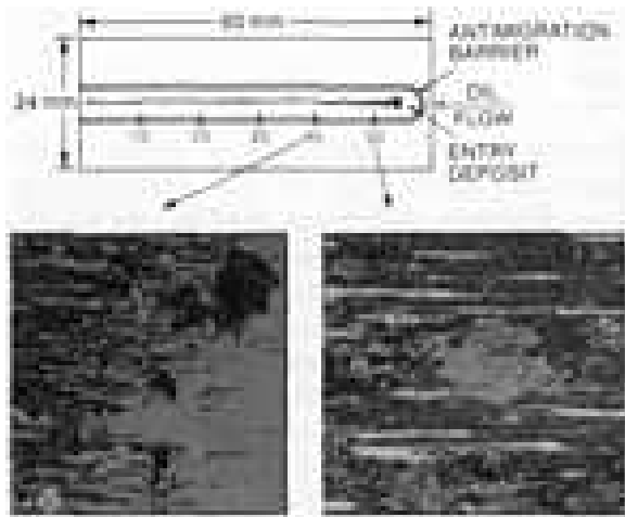
Fig. 3 Typical analytical ferrograph deposit patterns
