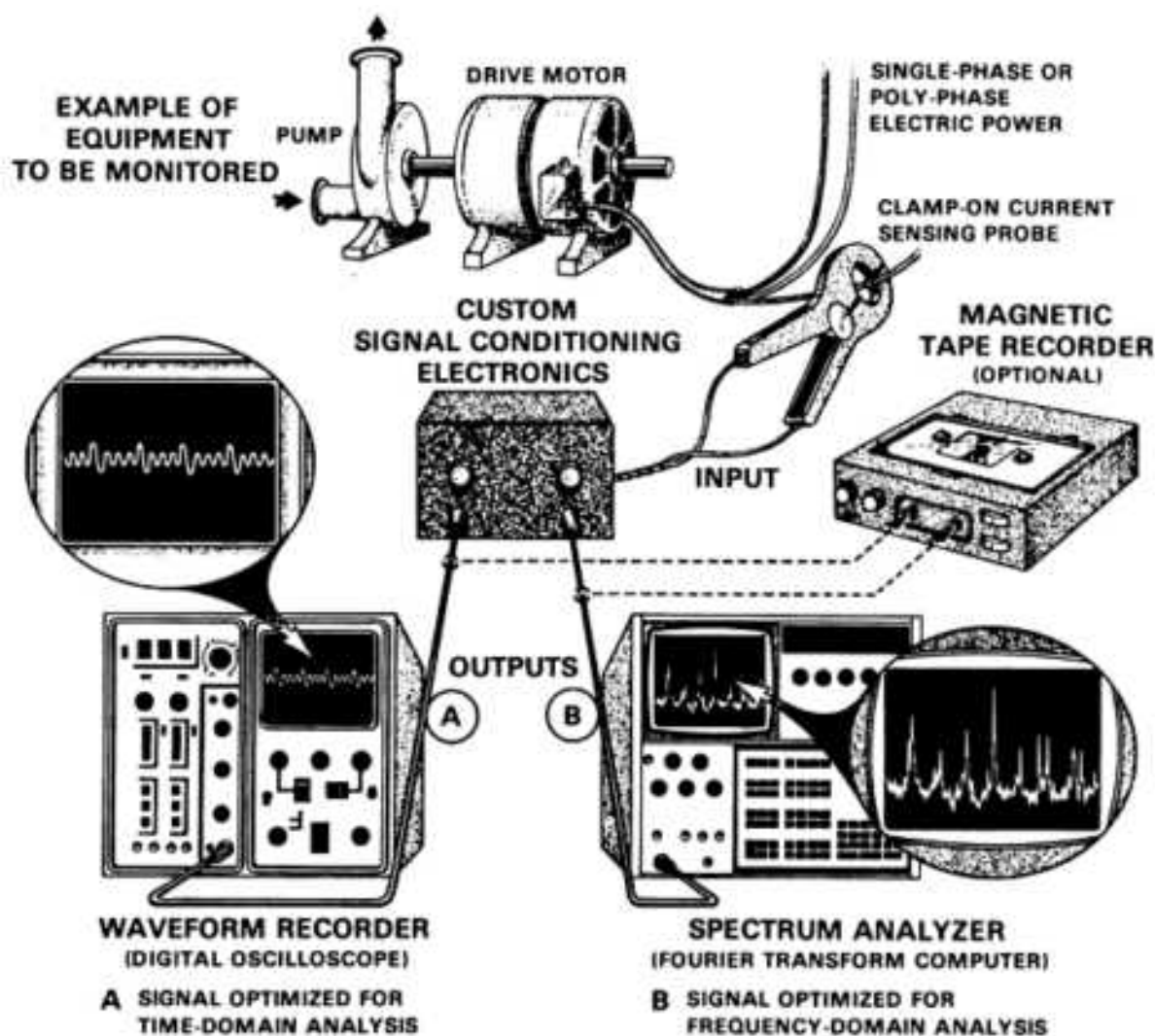
Fig. 2 Motor-current signature analysis (MCSA) method
