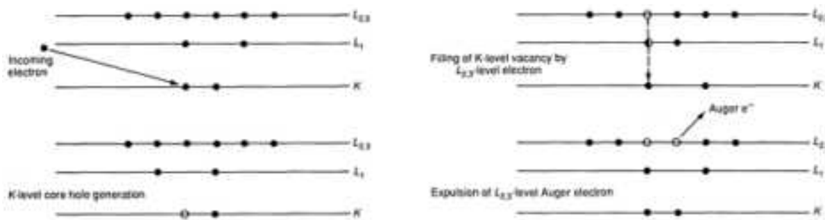
Fig. 13 Energy-level diagram at Auger KL_{2,3}, L_{2,3} electron emission process
