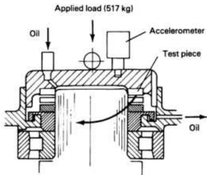
Fig. 4 Unisteel RCF testing apparatus. See Table 1.
