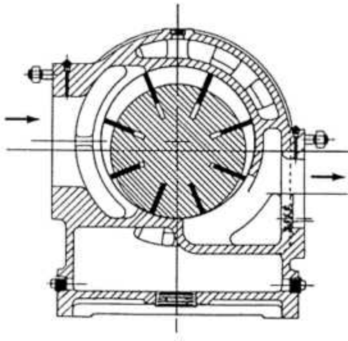
Fig. 11 Cross section of sliding vane compressor. Courtesy of AC Compressor Corporation.
