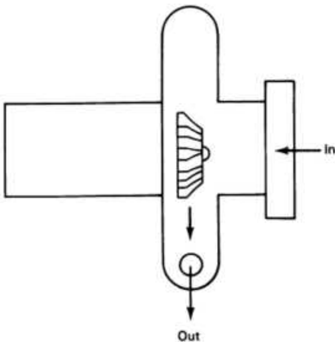
Fig. 12 Single-stage compressor
