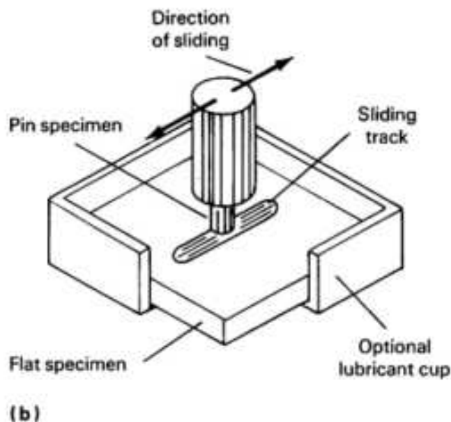
Fig. 11 Pin-on-disk wear test apparatus. (a) Key components of the device. (b) Close-up showing pin motion relative to flat when subjected to load. Source: Ref 2
