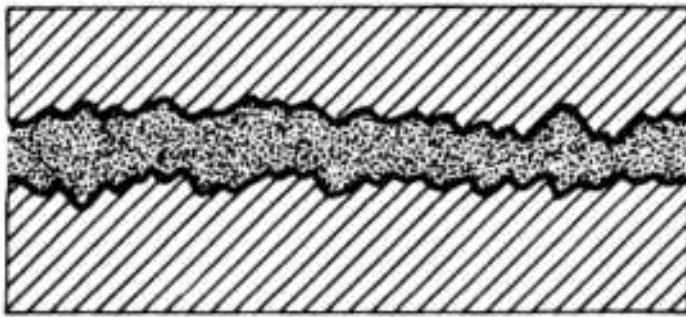
Fluid film lubrication — surfaces separated by bulk lubricant film
