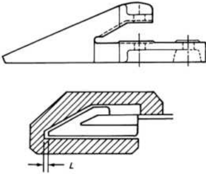
Fig. 5 Worn bucket tooth showing linear wear loss of amount L . Source: Ref 5
