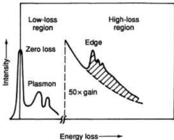
Fig. 23 Schematic illustration of EELS spectrum
