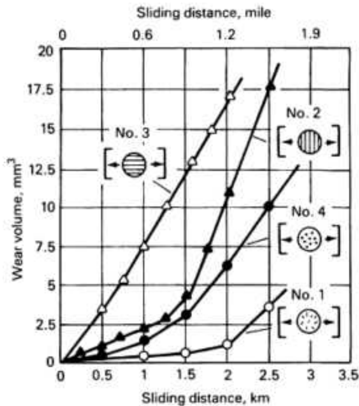
Fig. 20 Effect of sliding direction and fiber arrangement on wear volume of copper-carbon composite. P = 4.9 MPa (0.7 ksi)
