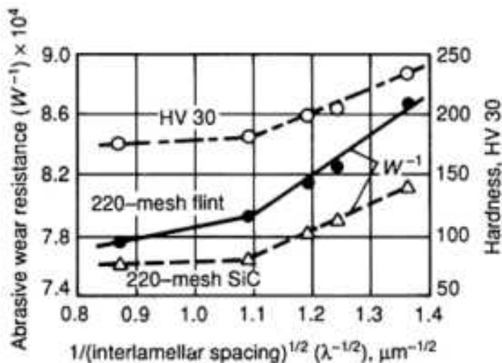
Fig. 9 Abrasive wear resistance and bulk hardness of 0.7% C steel as a function of pearlite interlamellar spacing. Abrasion data obtained using pin abrasion test apparatus with pressure, P , of 710 kPa (105 psi); two different 220-mesh abrasives (flint [96 to 99% Si] and silicon carbide) used in separate tests. Source: Ref 6
