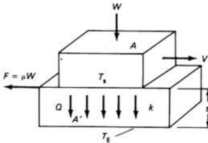
Fig. 2 Schematic showing parameters that affect frictional heat dissipated by conduction. Q , heat generated by friction; A' , area of larger rectangle; k , thermal conductivity; T_s , surface temperature; T_E , temperature of environment
