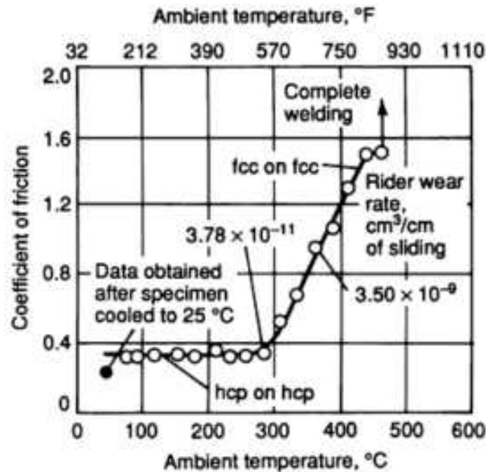
Fig. 10 Plot of coefficient of friction versus temperature as a function of phase transformation in a vacuum for cobalt sliding on cobalt. Sliding velocity, 1.98 m/s (6.5 ft/s). Source: Ref 19
