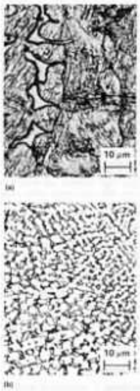
Fig. 9 Microstructures of laser-alloyed 1018 steel. (a) Addition of 16% Cr. (b) Addition of 43% Cr and 4.4% C. Source: Ref 33
