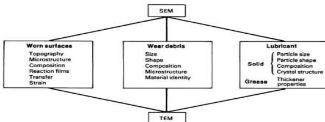
Fig. 1 Three different facets of wear to which SEM and TEM are applied
