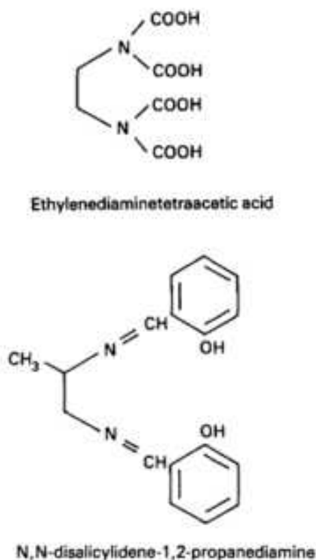
Fig. 14 Metal deactivators
