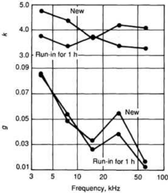
Fig. 11 Detecting the progress of "running in"
