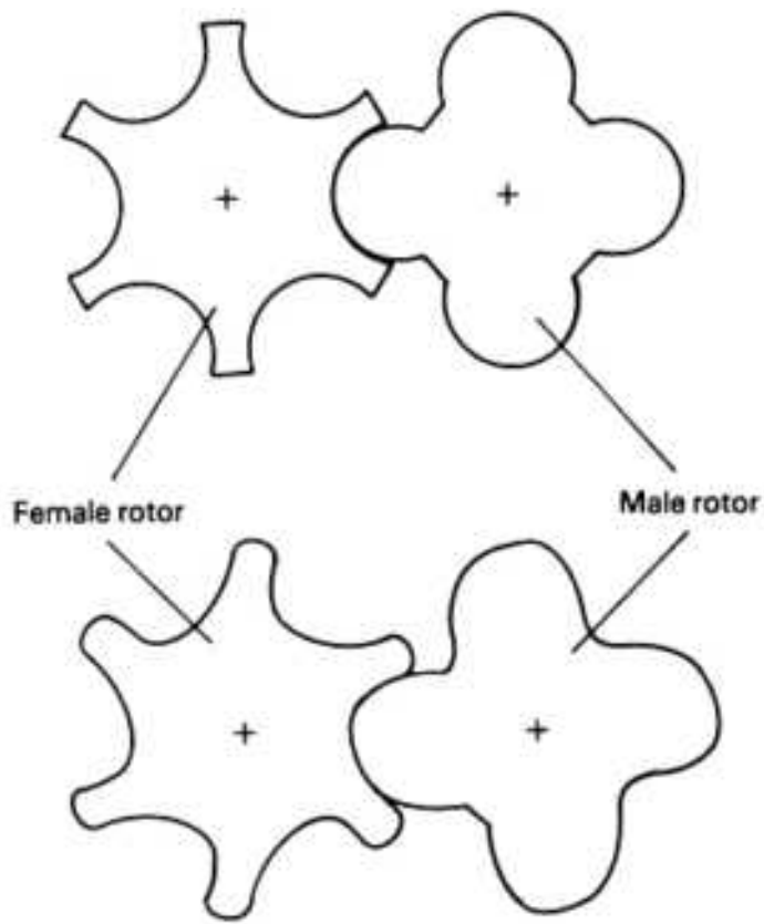
Fig. 9 Rotor profiles
