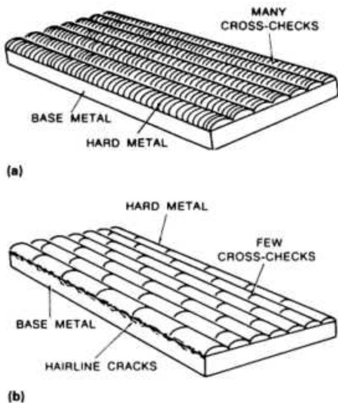
Fig. 14 (a) Sufficient cross-checks. (b) Insufficient cross-checks. Source: Ref 32
