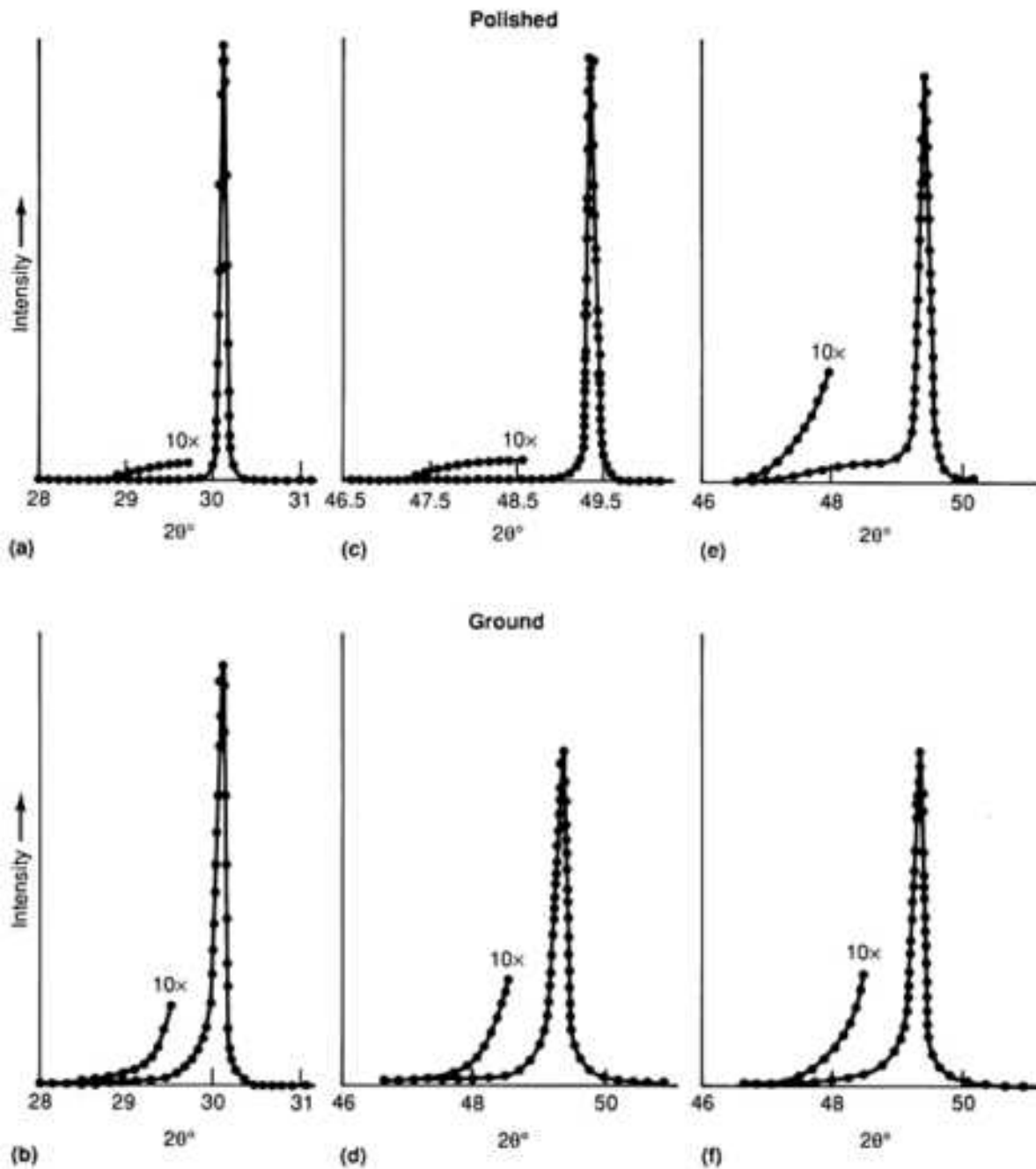
Fig. 8 (111) intensity bands from polished and ground samples of partially stabilized zirconia showing experimental data points and computer simulations (solid lines) for and symmetrical optics with CuK \alpha radiation ( \lambda - 0.15406 nm), (a) and (b); synchrotron radiation with \lambda = 0.24797 nm, (c) and (d); and 3° asymmetric optics with \lambda = 0.24797 nm, (e) and (f)
