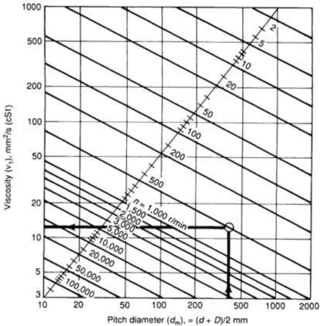
Fig. 4 Calculation of minimum required viscosity
