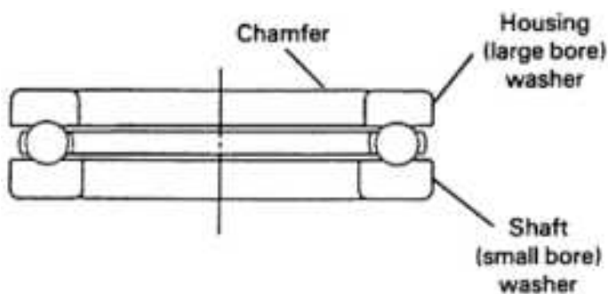
Fig. 8 Thrust ball bearing designed to carry axial load only due to 90^\circ contact angle
