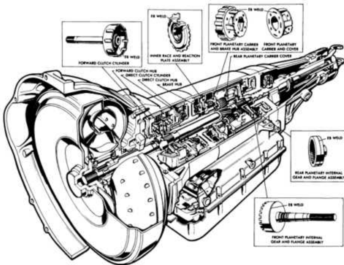
Fig. 1 Borg-Warner Model 12 automatic transmission. EB, electron beam
